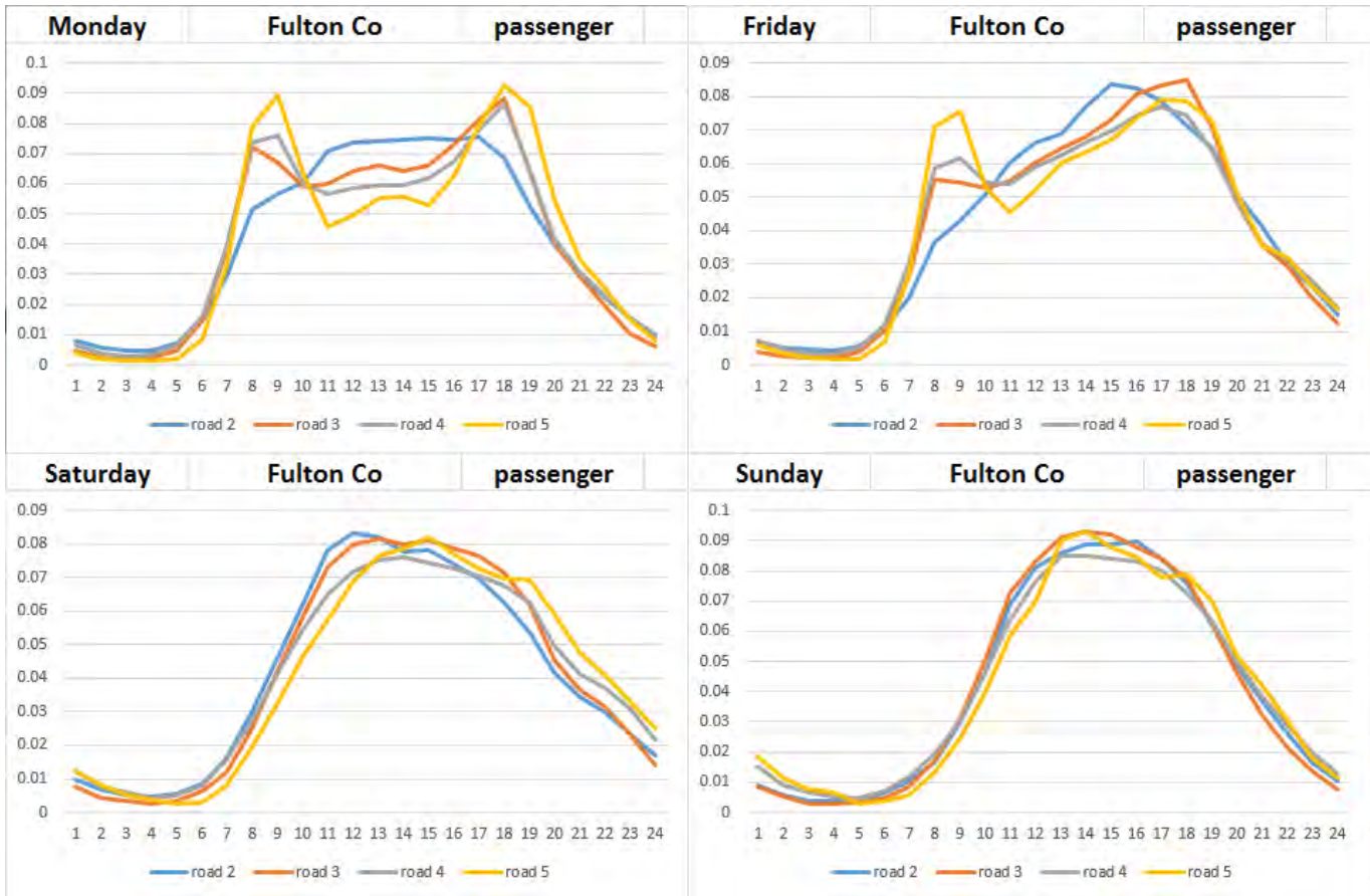
Figure 3-25. Sample onroad diurnal profiles for Fulton County, GA
