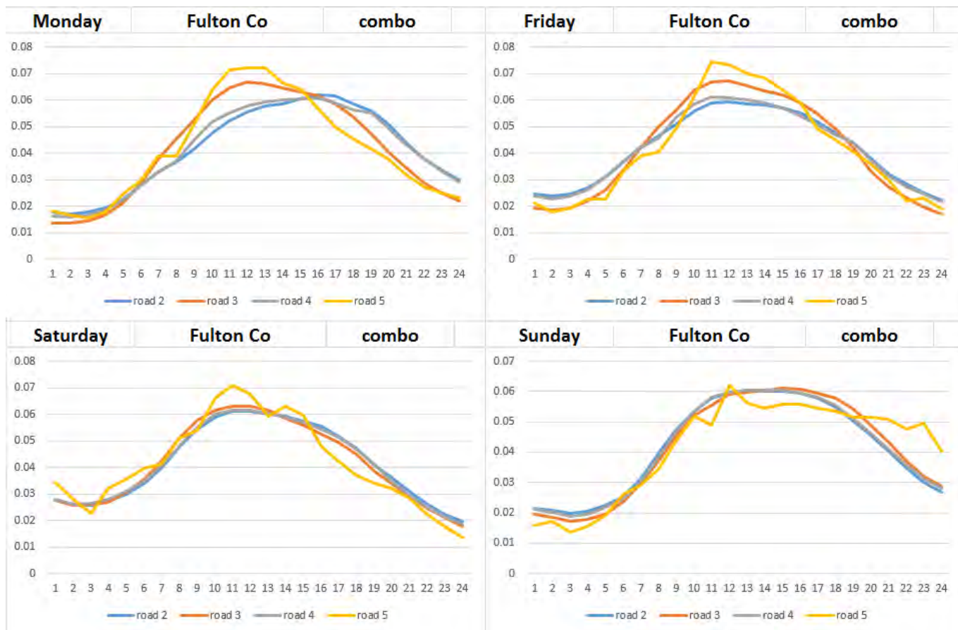
Figure 3-28. Example of Temporal Profiles for Combination Trucks
