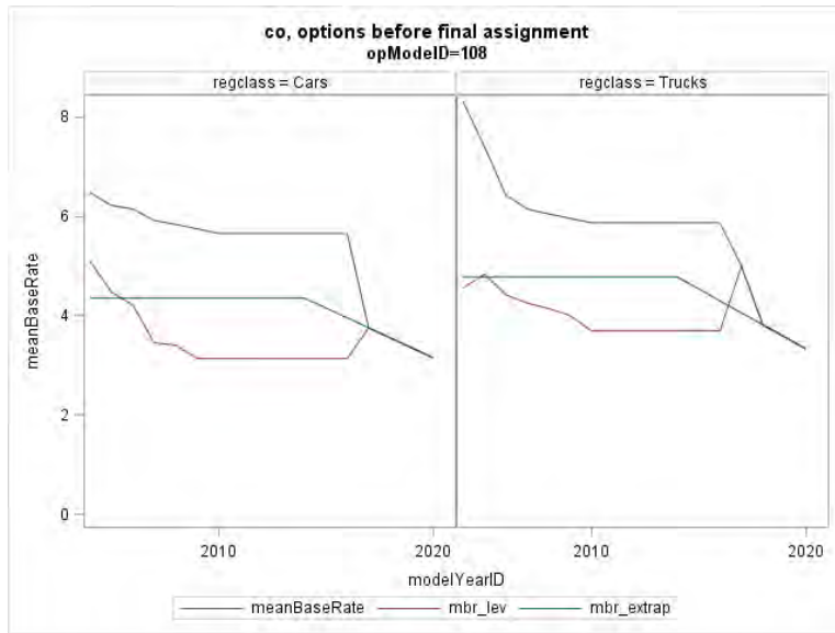
Figure 3-128 CO: Trends in Emissions for Federal and Estimated CA/S.177 rates, for cars and trucks at age 0-3 years, for the start emissions process (opModelID = 108)
