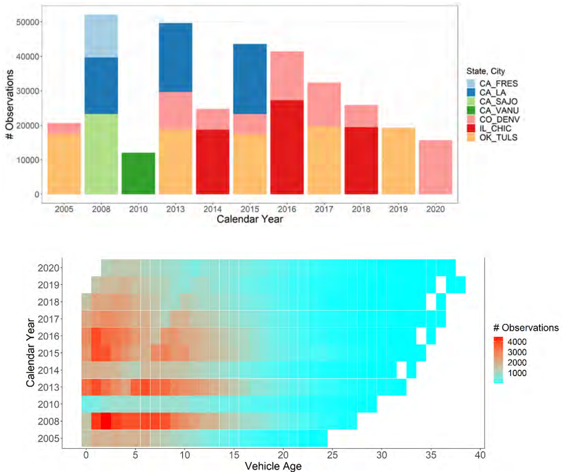
Figure 6-1. Top panel: Number of Vehicle Ammonia Measurements by Location and Calendar Year. Bottom panel: Number of Vehicle Ammonia Measurements by Vehicle Age and Calendar Year
