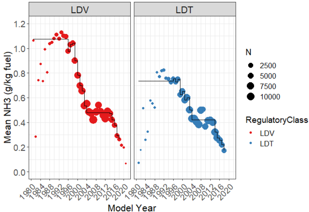
Figure 6-2. Average fuel-specific emission rates for light-duty vehicles (LDV) and light-duty trucks (LDT) by model year. The size of the points corresponds to the number of vehicle observations. The line is the average emission rate using the model year averaging specified in Table 6-3
