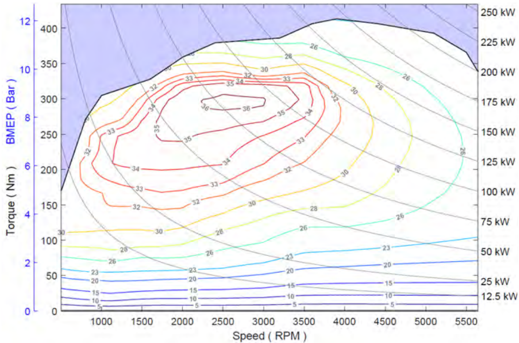
Figure 3-69: 2014 Chevrolet 4.3L EcoTec3 LV3 Engine LEV VIII Fuel - Cylinder Deactivation BTE (%) (U.S. EPA 2023b).
