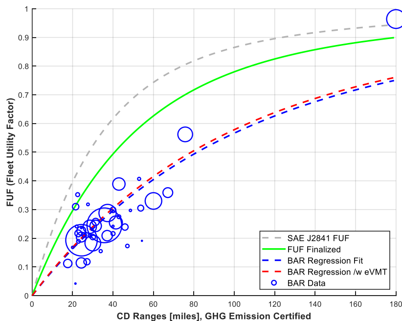
Figure 3-49. FUF Regression Fits with CD engine-on blended mode eVMT distance
