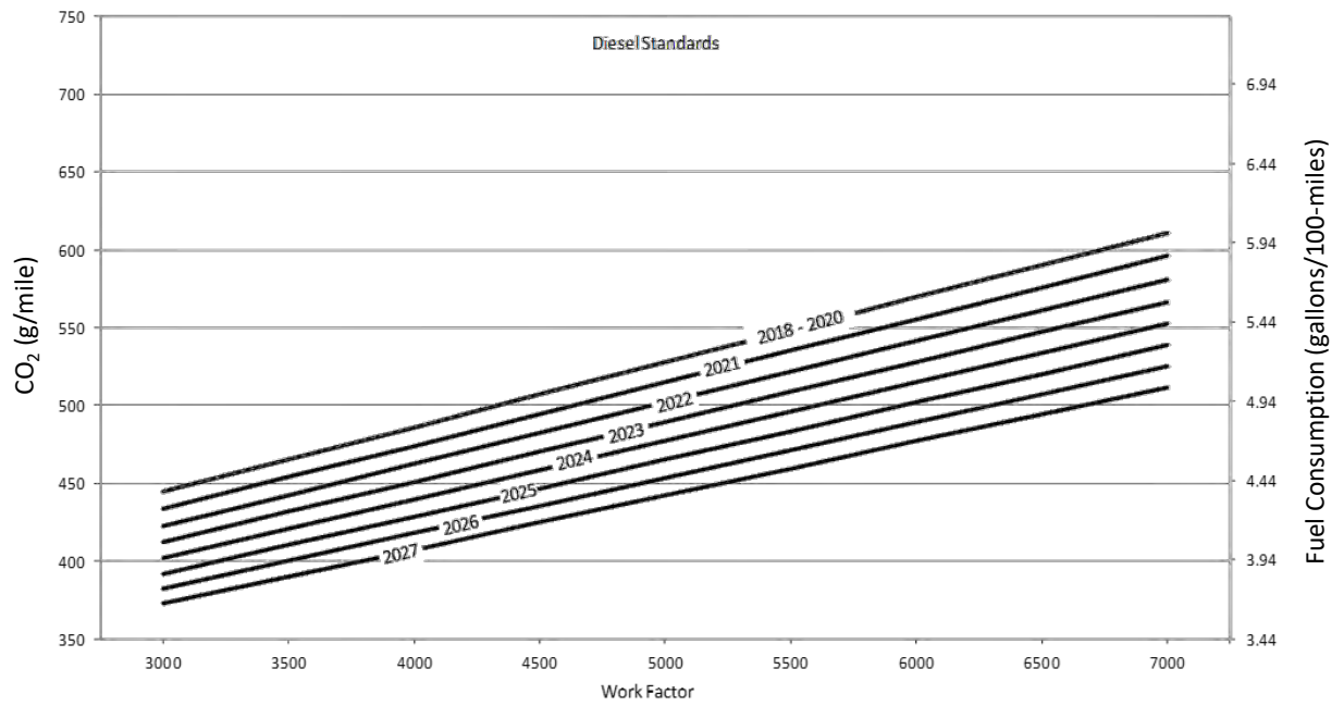
Figure 1-15: Heavy-duty Phase 2 work factor-based GHG standards for medium-duty pickups and vans (81 FR 73478 2016).
