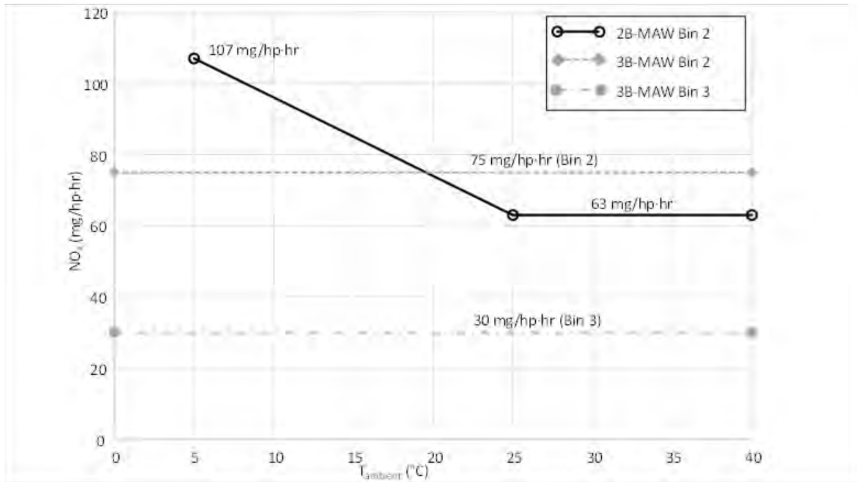
Figure 3-16: Figure 8: 2B-MAW Bin 2 In-use NO x standard with Ambient Temperature Correction and PEMS Accuracy Margin Compared to 3B-MAW Bin 2 and Bin 3 In-use NO x standard.
