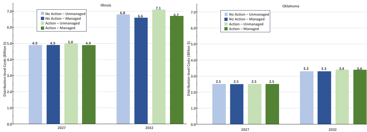
Figure 5-26: A comparison of the costs needed for distribution level upgrades for the no-action and action scenarios and showing the impacts of managed vs. unmanaged charging in Illinois (left) and Oklahoma (right).
