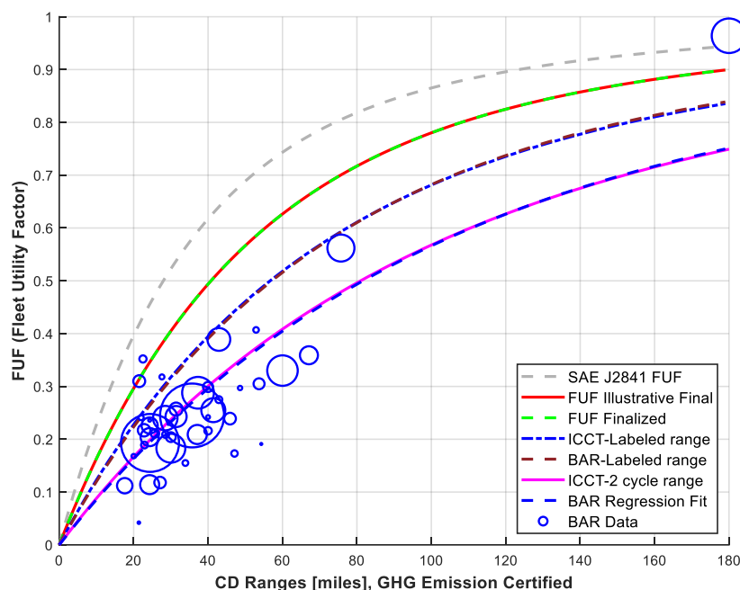
Figure 3-50: The Finalized FUF, SAE FUF, and ICCT Curves on 2-cycle combined GHG emission-certified CD range
