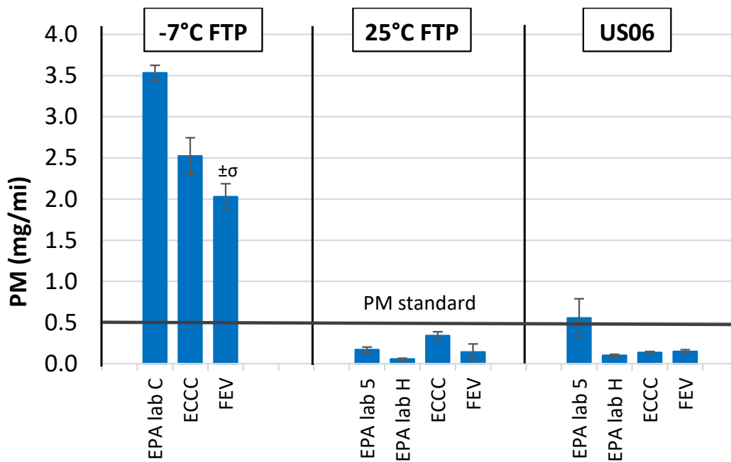
Figure 3-30: Test-to-test and lab-to-lab variability for 2021 Corolla.
