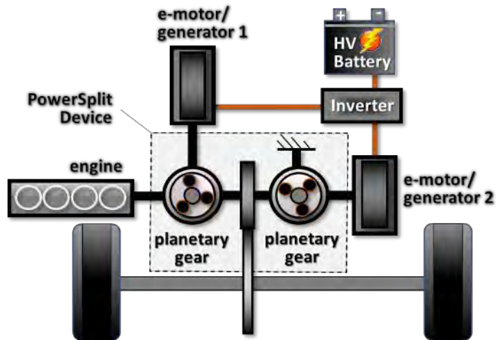
Figure 2-7: PowerSplit strong HEV and PHEV (& planetary gear arrangement).
