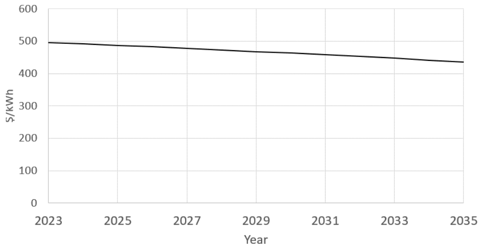
Figure 2-27: Ni/Mn HEV battery pack direct manufacturing cost (1.5 kWh example).
