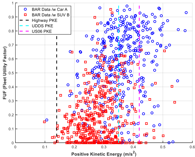
Figure 3-47. FUF vs. Positive Kinetic Energy
