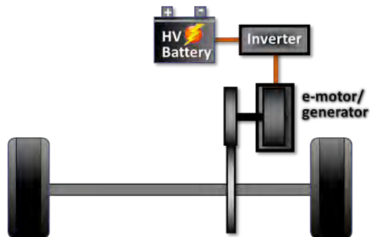
Figure 2-11: Battery electric vehicle architecture.
