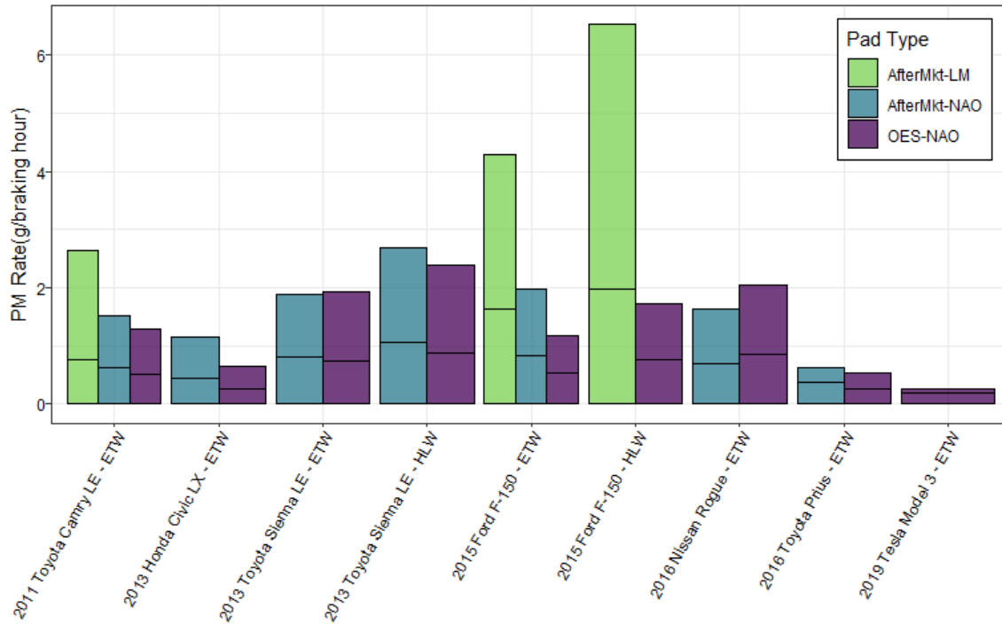
Figure 2-5 Vehicle-level emission rates for each vehicle and pad configuration tested. Each bar represents the PM 10 rate for the test configuration. The horizontal lines within each bar indicate the PM 2.5 rate.
