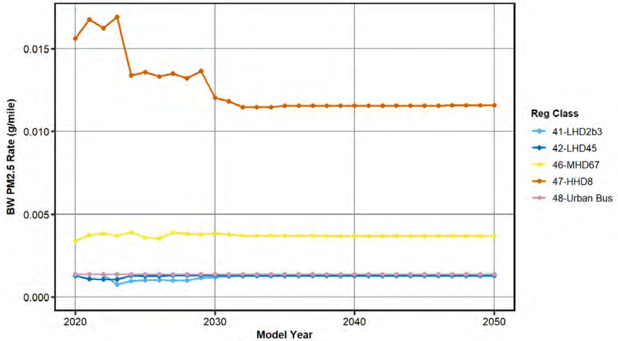
Figure 2-20 Brake wear PM 2.5 emission rates for heavy-duty electric vehicles averaged over a nationally representative operating mode distribution
