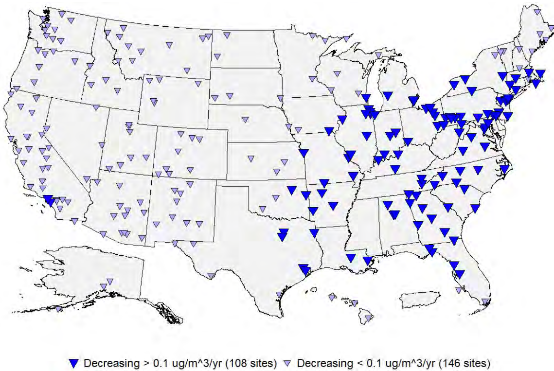
Figure 2-32. Trends in annual average concentrations for sulfate (SO 4 2- ) from 2006 through 2021.
