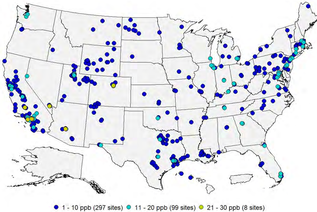
5 6 Figure 2-19. Primary and secondary NO 2 design values (single year annual mean; ppb) 7 for 2021.
