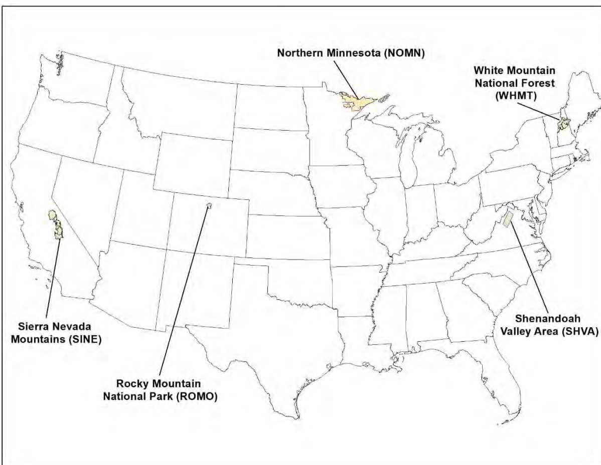
Figure 5A-52. Location of the case study areas. Northern Minnesota (NOMN), Rocky Mountain National Park (ROMO), Shenandoah Valley (SHVA), Sierra Nevada Mountains (SINE) and White Mountain National Forest (WHMT).
