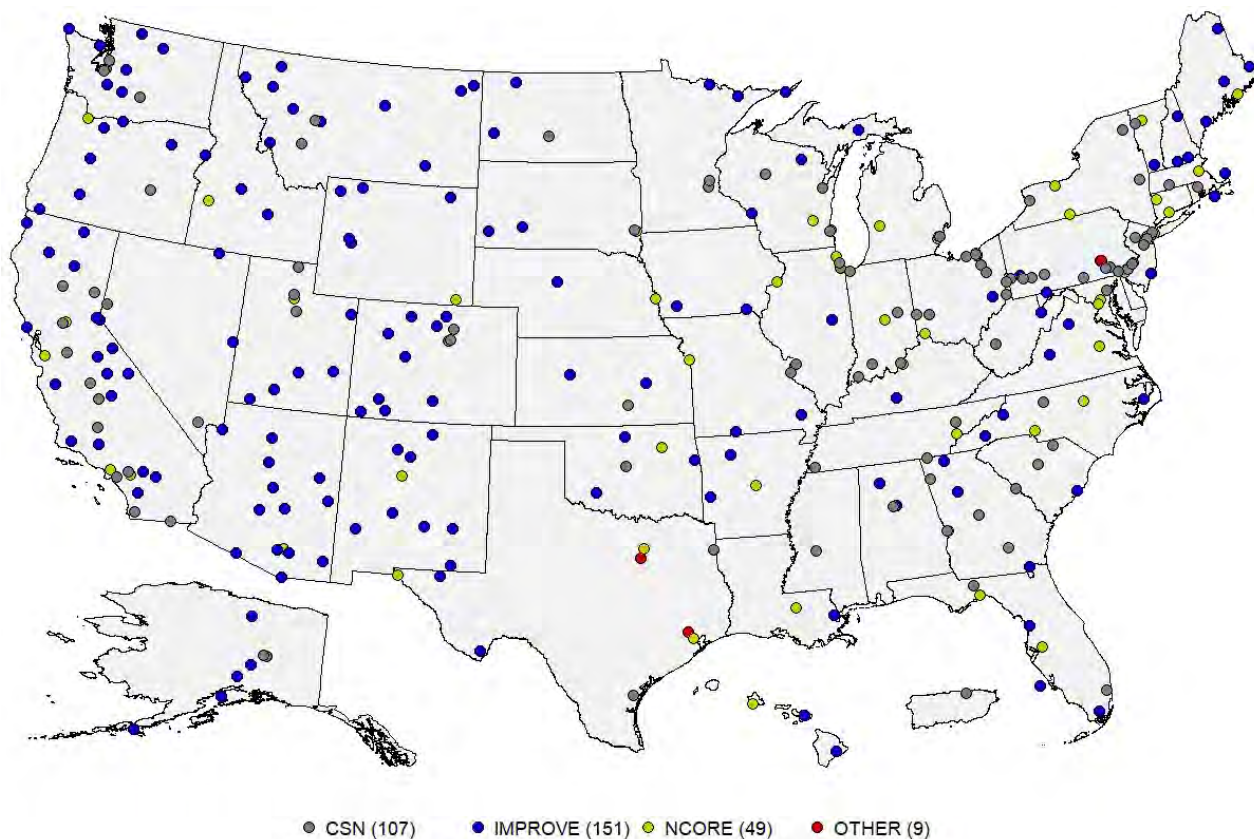
2 Figure 2-14. PM 2.5 speciation monitors operating during the 2019-2021 period.
