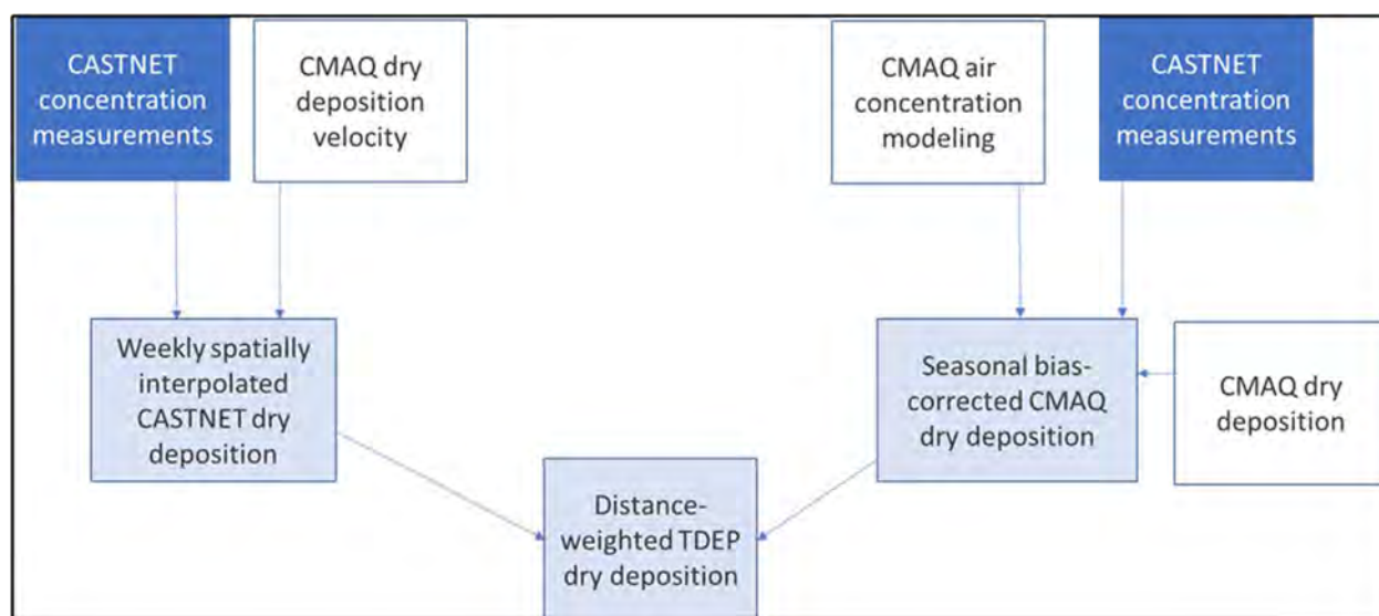
7 Figure 2-37. Data sources for estimating dry deposition. Dark blue indicates observations, 8 white boxes indicate chemical transport modeling results, and light blue boxes 9 are the results of model-measurement fusion. Note that the bias correction is not 10 applied to ammonia, in part, because the existing method must be modified to 11 account for its bidirectional flux.
