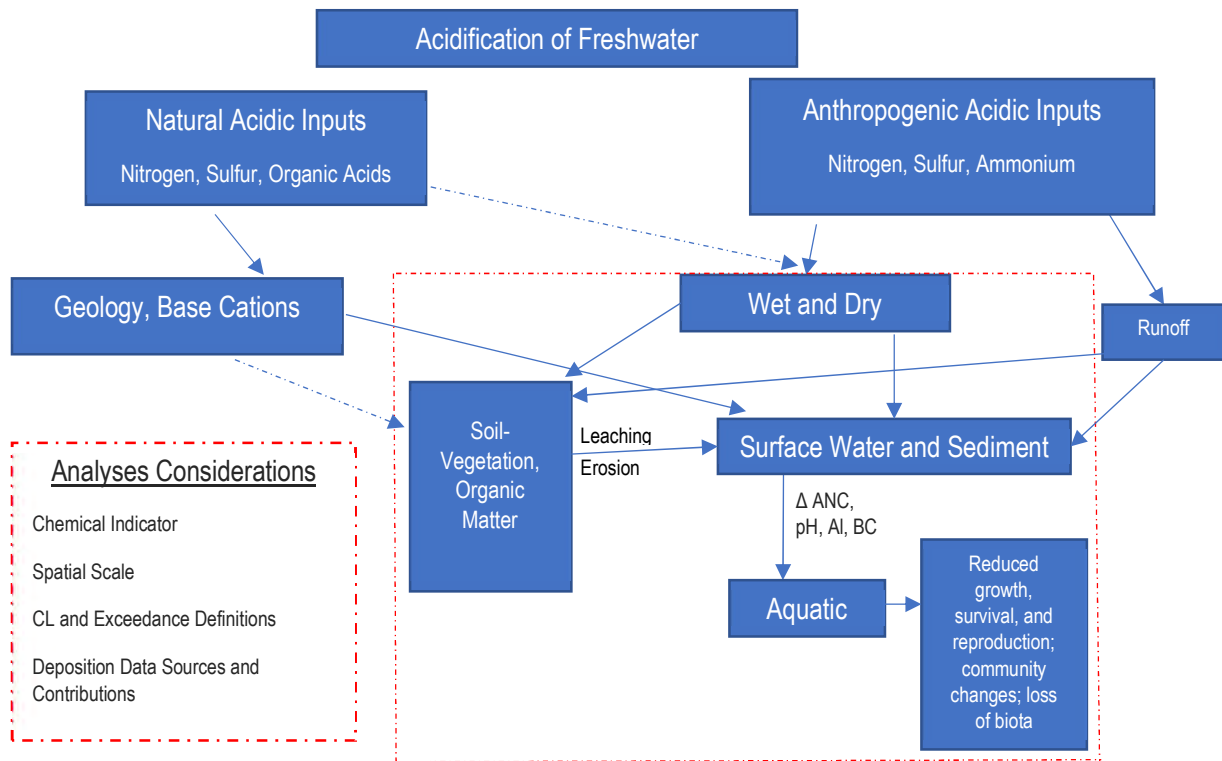
16 17 Figure 5-4. Conceptual Model for Aquatic Acidification Analyses
