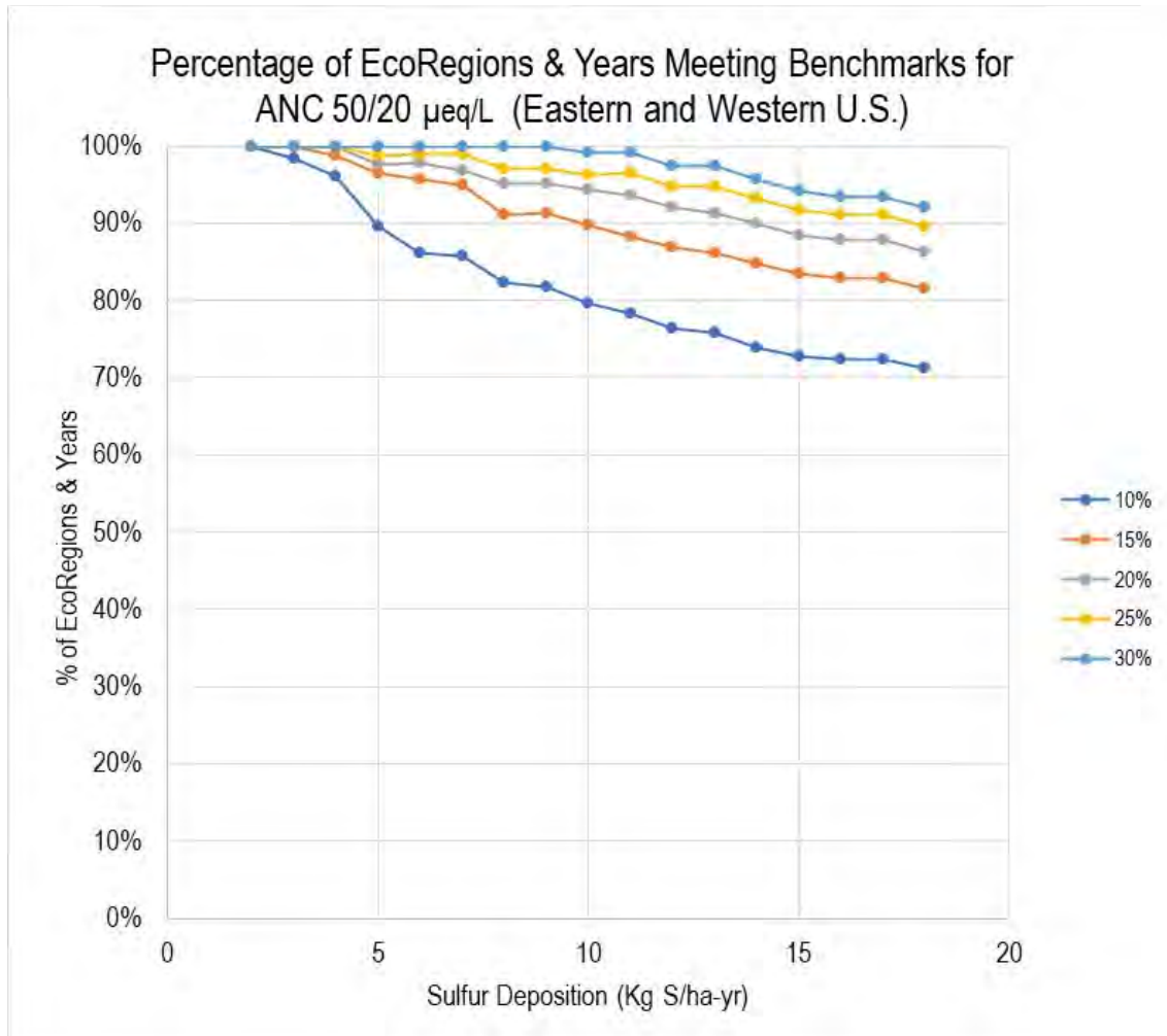
Figure 5A-48. Cumulative percent of ecoregions with exceedances >10, >15, >20, >25, >30% as a function of total S deposition across all 5 deposition periods (2001-03, 2006-08, 2010-12, 2014-06, 2018-20). 100% indicates there were no ecoregion that had percent exceedances above >10, >15, >20, >25, >30% for a given deposition level. Critical load exceedances based on ANC threshold of 50 µeq/L for the east and 20 µeq/L for the west (50/20 µeq/L) (See Table 5A-35 for data).
