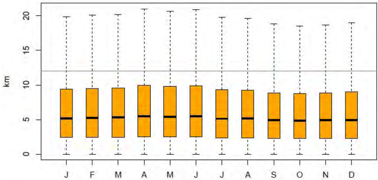
Figure 3.1.6. Distribution of hourly wind displacement by hour and month.
