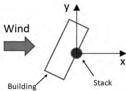
Figure 3-2. Fixed Stack location with respect to Building and Wind Flow Orientation
