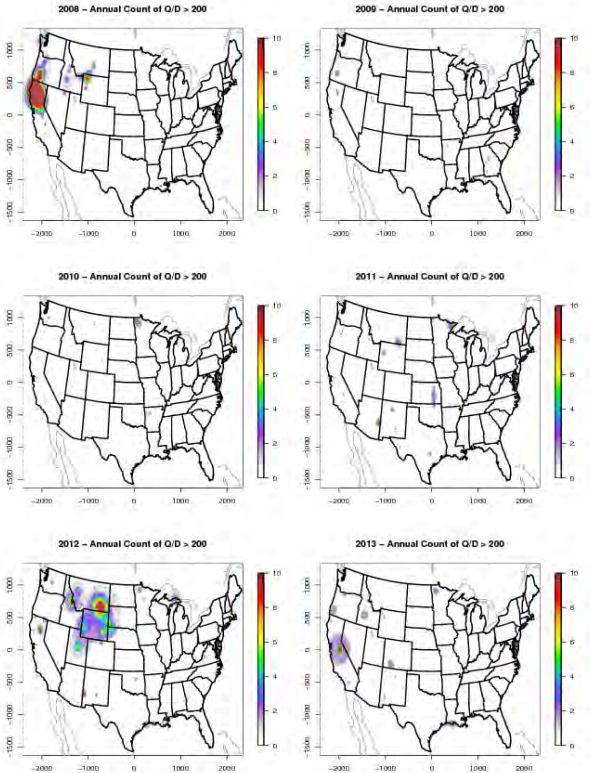
Figure A2-8. Count of days with \text{NO}_x + \text{rVOC} Q/D > 200 for 2008 through 2013. Note scale has been capped at 10 to more easily distinguish the values below 10. Red may actually indicate 10 or greater than 10.
