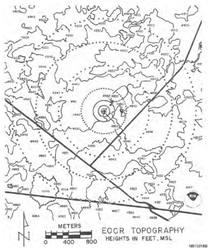
Figure 6. Terrain map featuring the entire EOCR grid with the source at the grid center ( \text{SF}_6 releases). Arcs are at distances of about 40, 80, 200, 400, 800, 1200, and 1600 m.
