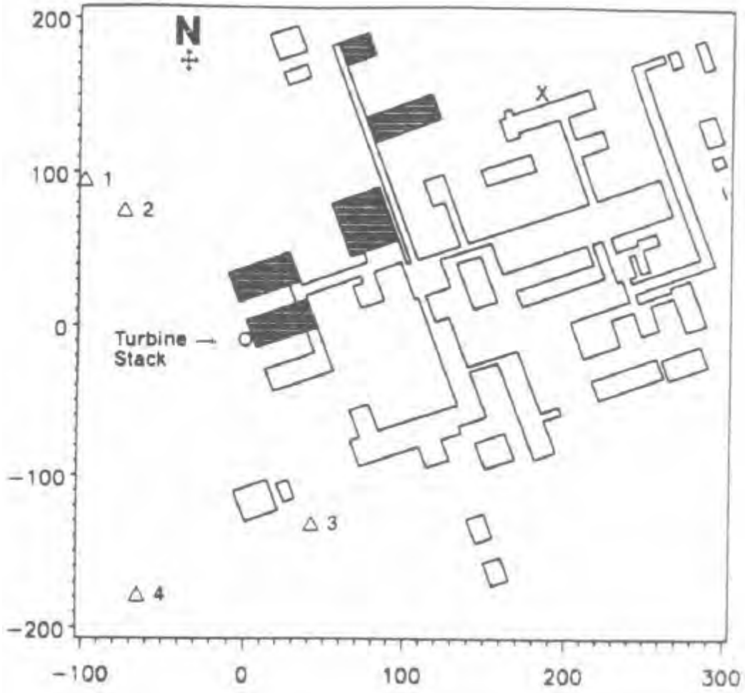
Figure 7. Depiction of Alaska North Slope Oil Gathering Center turbine stack, meteorological tower (X), and camera locations used to visualize plume rise.
